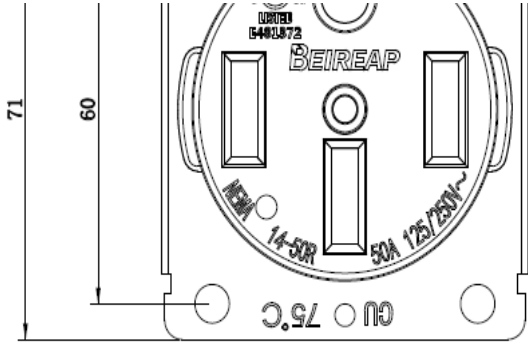
Dimension & Assembly drawing
